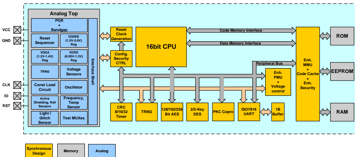
Fig. 1.1: Block Diagram
